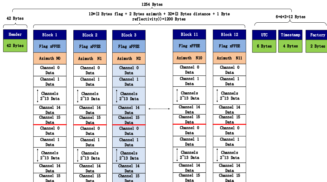
Figure 5.1 Data Format of the Single Echo Mode
