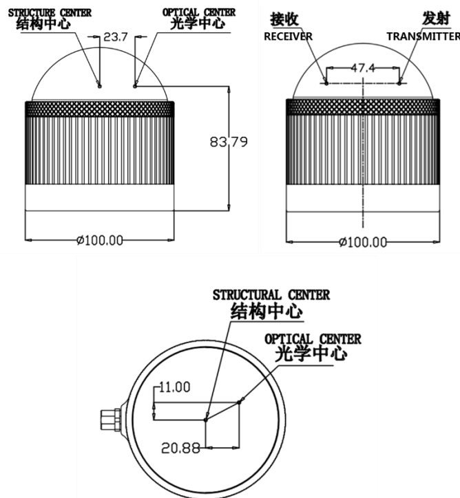
Figure 1.4 CH16R Mechanical Drawing (unit: mm)
