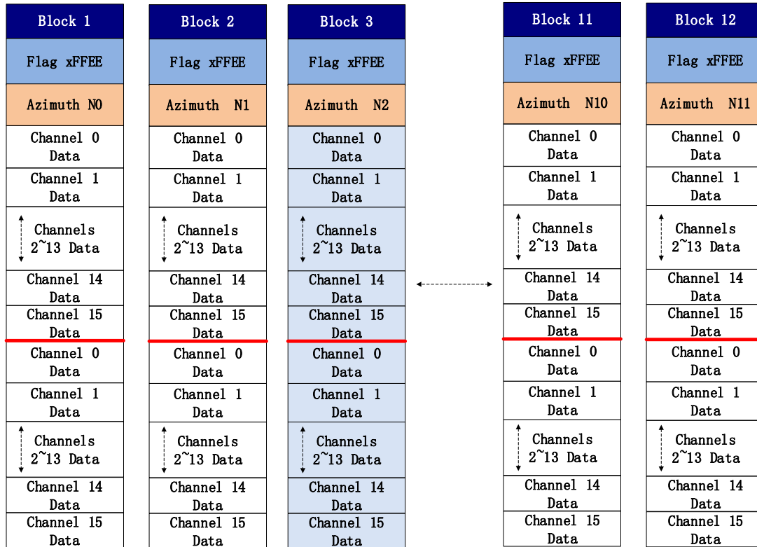
Figure 7.1 Single Echo Data Block Structure
