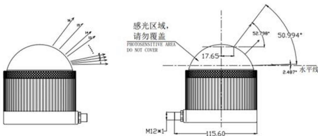
Figure 1.2 Laser Beam Distribution
