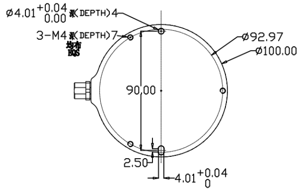
Figure 1.5 CH16R Lidar Base (unit: mm)
