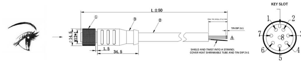
Figure 2.4 CH16R Lidar Extension Cable (unit: mm)
